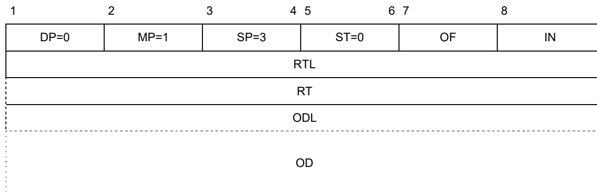
Figure 5-19. ROUTE packet
