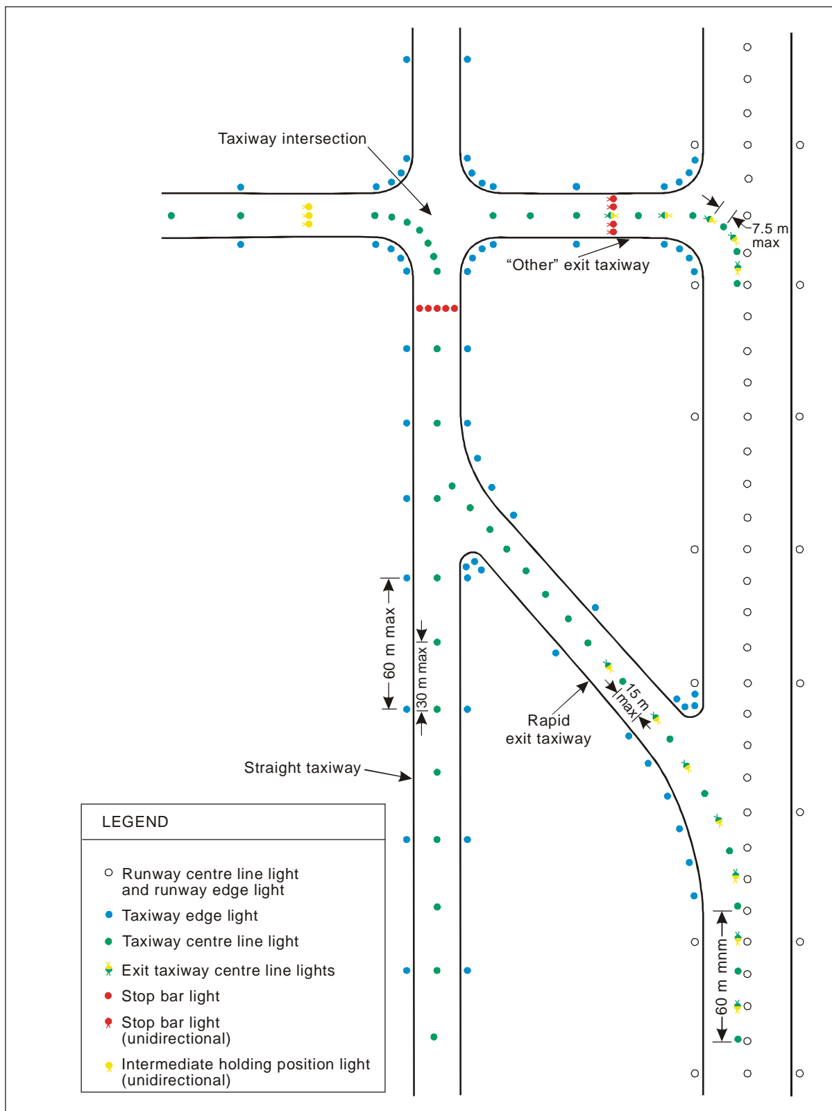
Figure 5-26. Taxiway lighting
