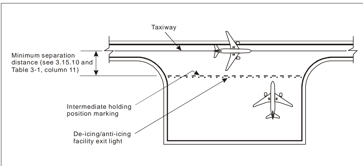
Figure 5-28. Typical remote de-icing/anti-icing facility
