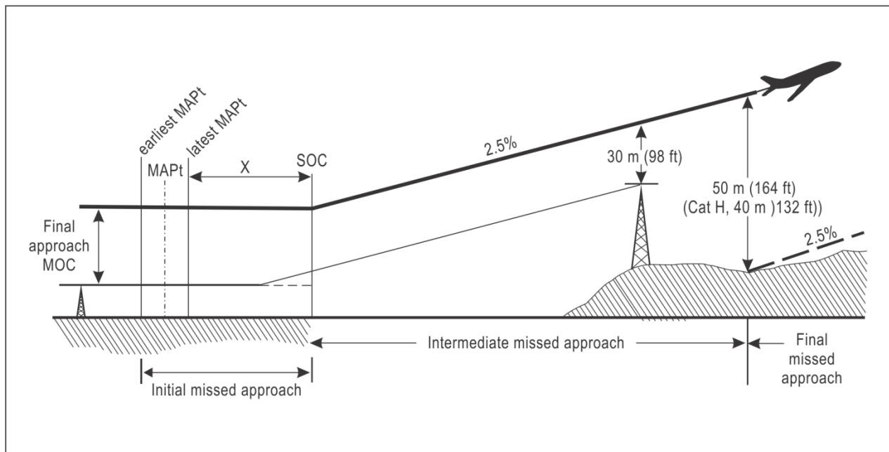
Figure A-3-1. Obstacle clearance in the missed approach
