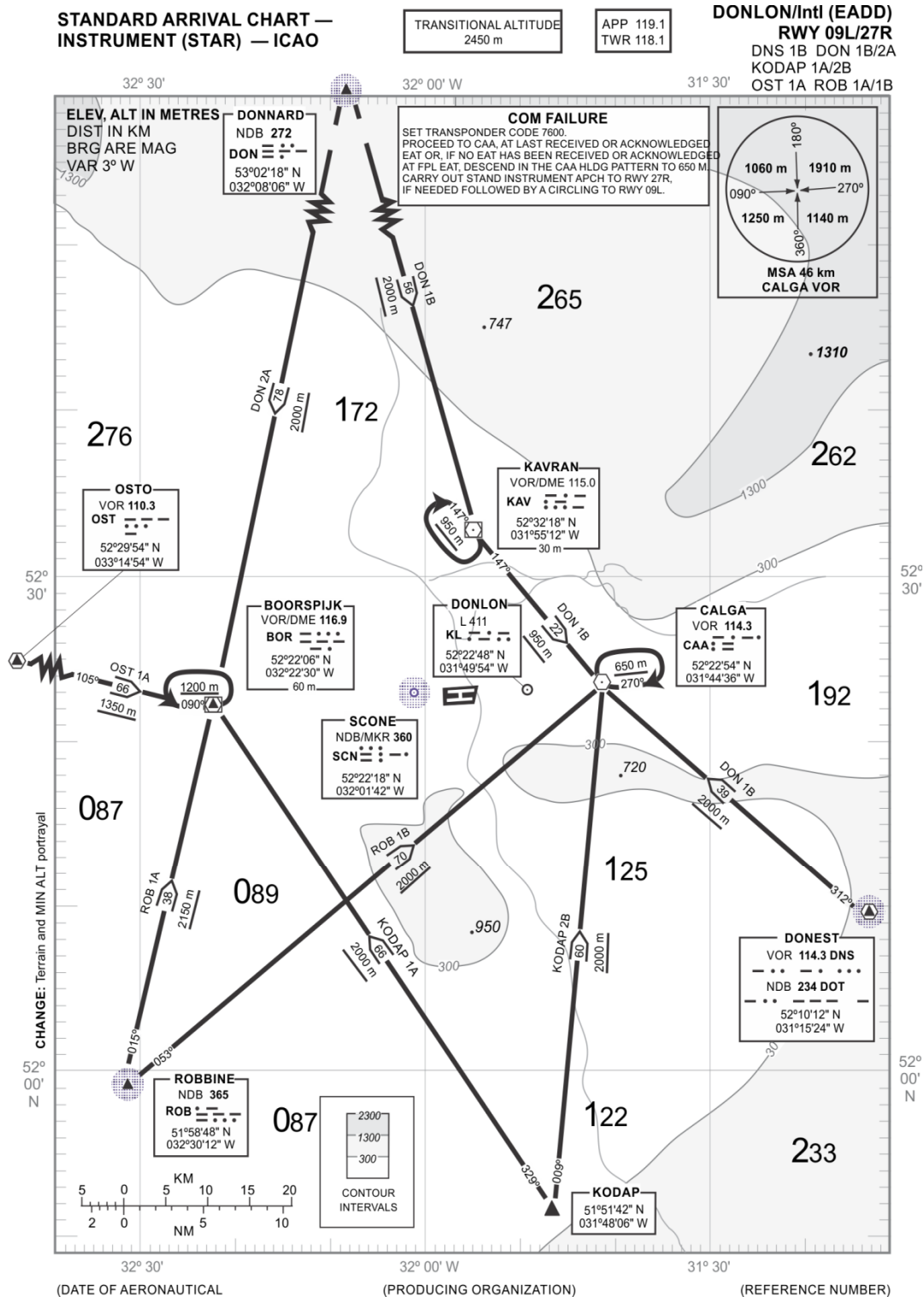
Sample Chart 2. Standard instrument arrival (STAR)
