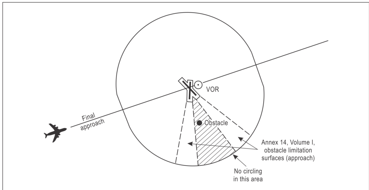
Figure II-5-6-2. Visual manoeuvring (circling) area — prohibition on circling
