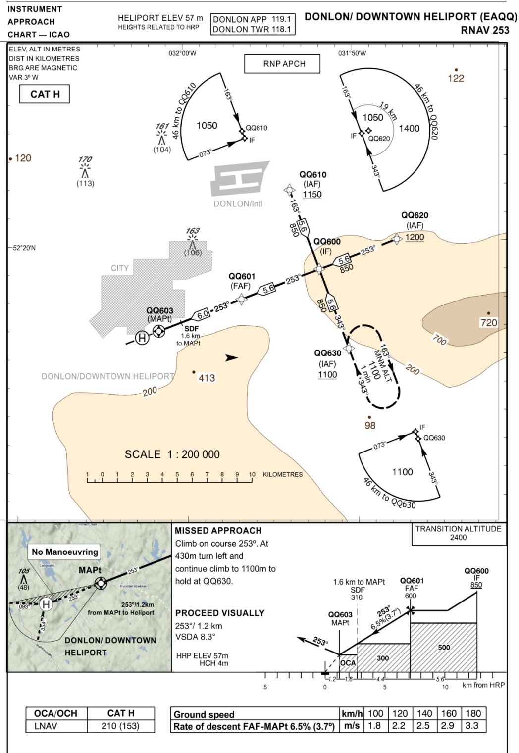
Sample Chart 8. Helicopter PinS approach to LNAV minima ("proceed visually")
